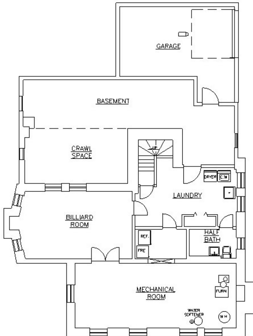
70 Monte Vista Ave Basement Floor Plan
