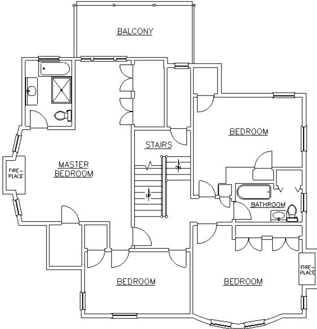
70 Monte Vista Ave 2nd Floor Plan
