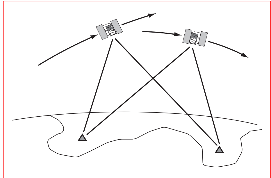
Double Differencing
