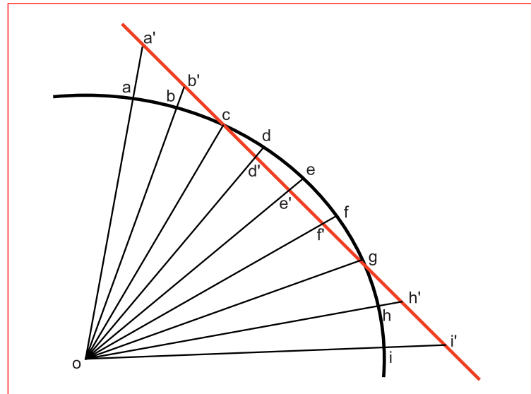
The basic idea behind map projections
